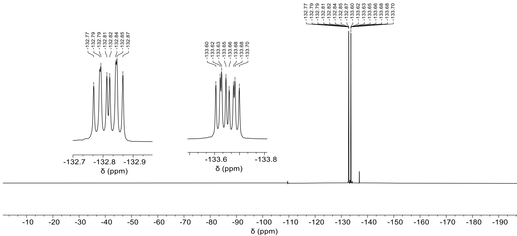
^{19}\text{F} NMR (377 MHz, \text{CDCl}_3 ) of 2,3,7,8-tetrafluorothianthrene-S-oxide (2).
